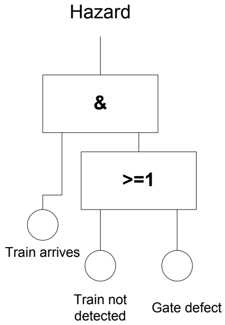
System (Fault Tree)
